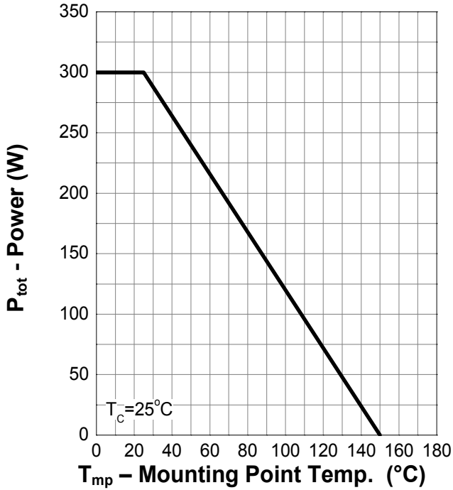
Power Capability
