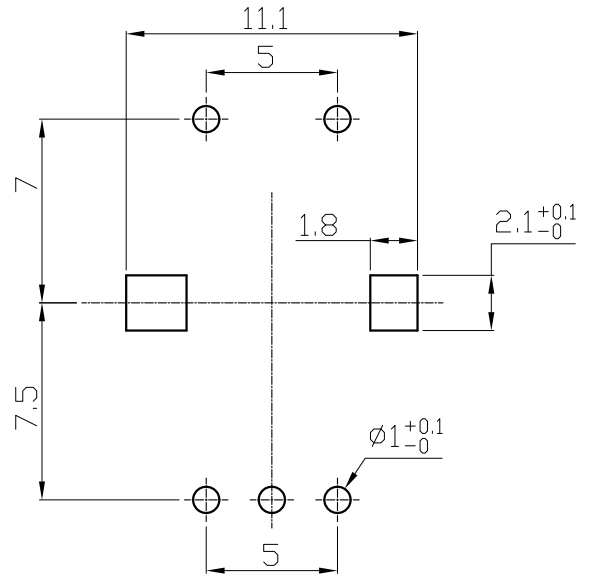
P.C.B.MOUNTING DETAIL
