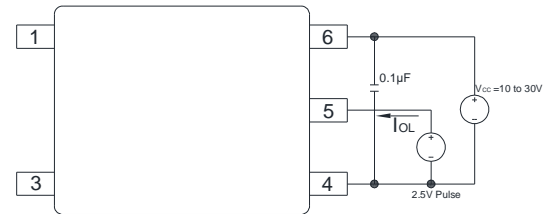
Figure 17 : I OL Test Circuit
