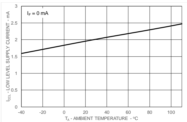
Figure 5. I_{CCL} vs. Temperature
