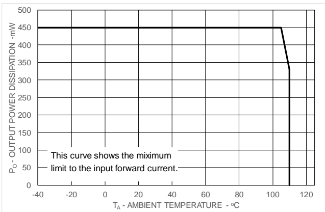
Figure 3. P_O vs. Temperature
