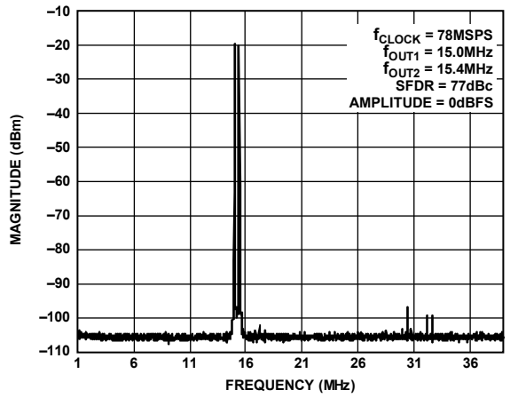
Figure 25. Dual-Tone SFDR
