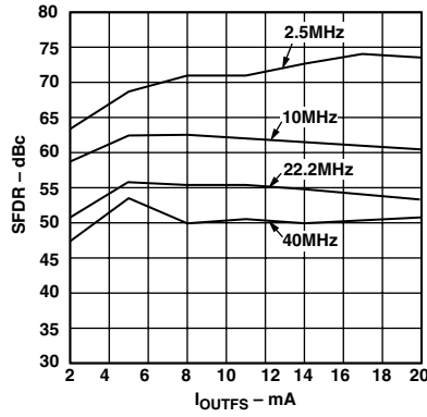
Figure 31. SFDR vs. f_{\text{OUT}} and I_{\text{OUTFS}} @ 100 \text{ MSPS} , 0 \text{ dBFS}
