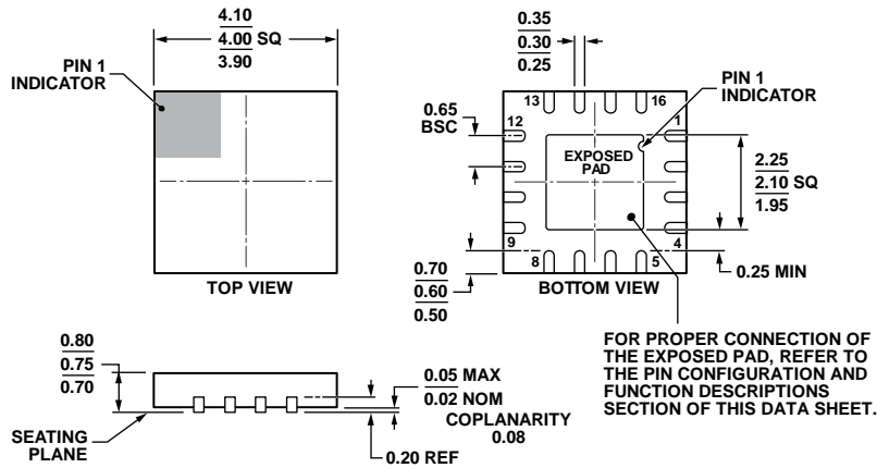
Figure 53. 16-Lead Lead Frame Chip Scale Package [LFCSP_WQ] 4 mm × 4 mm Body, Very Thin Quad (CP-16-23) Dimensions shown in millimeters
