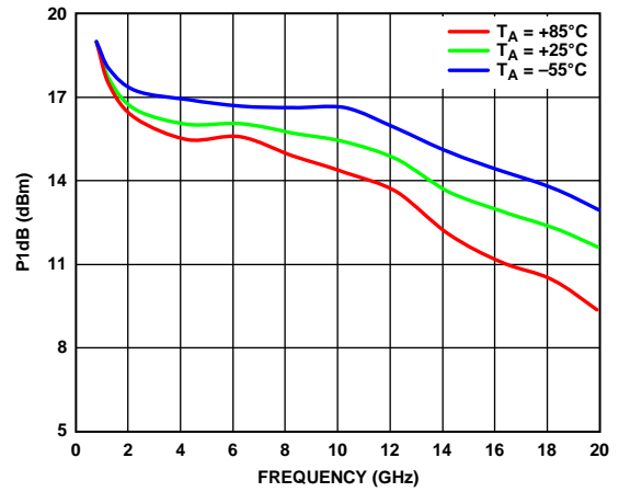
Figure 32. P1dB vs. Temperature
