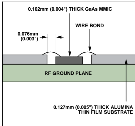
Figure 36. RF Lines
