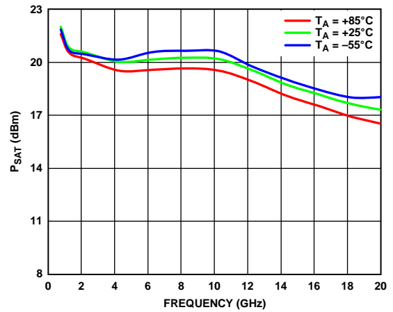
Figure 33. P_{SAT} vs. Temperature
