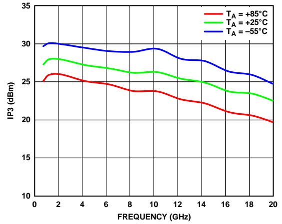
Figure 31. Output IP3 vs. Temperature
