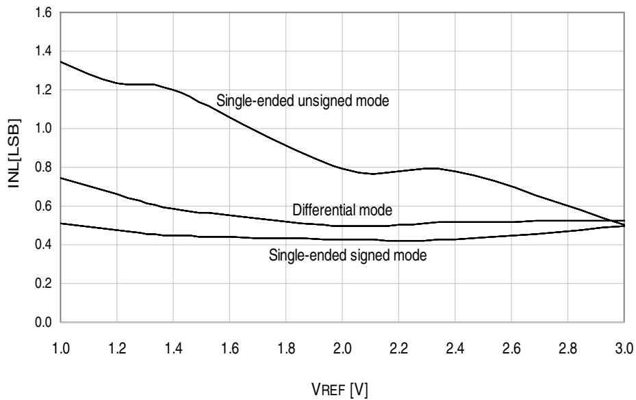
Figure 34-242. INL Error vs. External V_{REF}
