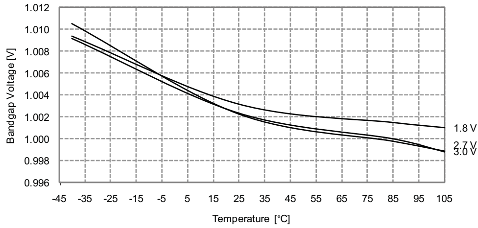
Figure 34-327. ADC Internal 1.0V Reference vs. Temperature
