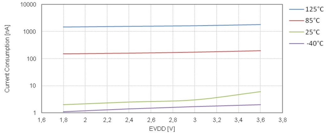
Figure B-11. Current Consumption in DEEP SLEEP.
