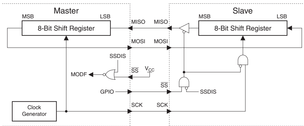
Figure 18-2. SPI Master-Slave Interconnection
