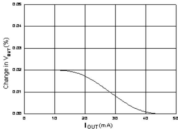
Figure 5 Load Regulation
