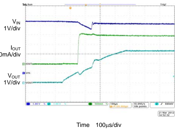
Figure 29. Leave OVP Function ( V_{IN} =6V to 5V)
