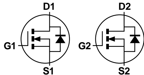
Equivalent Circuit
