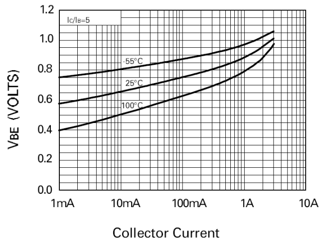
Collector Current V_{BE(SAT)} vs I_C
