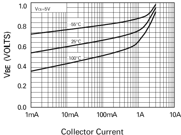
Collector Current V_{BE(ON)} vs I_C
