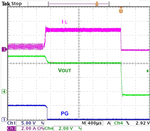
Figure 19. Overload Protection
