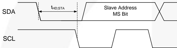
Figure 20. START Bit
