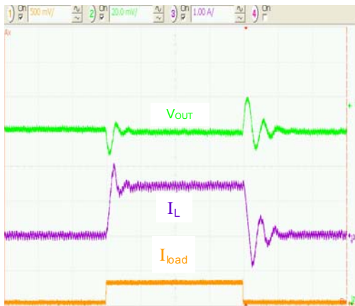
Figure 15. MODE=1, 100 mA to 1.5 A to 100 mA, 5 \mu\text{s}/\text{div} .
