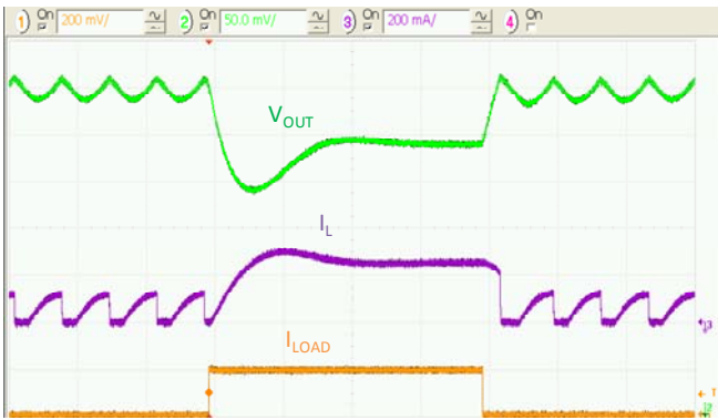
Figure 23. Load Transient 50mA to 250mA, V_{IN}=3V , t_{RISE}=t_{FALL}=100ns , 5\mu s/div .
