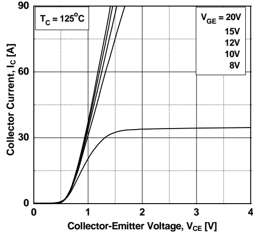
Figure 4. Transfer characteristics
