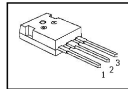
PG-TO247-3-1
