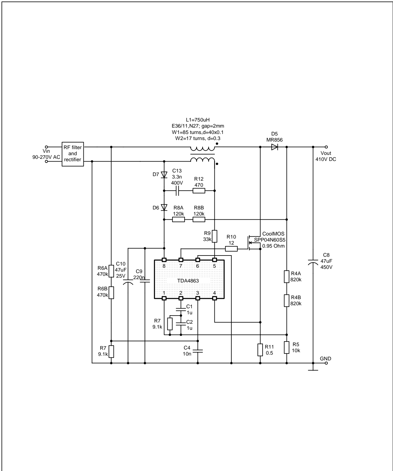
Figure 5 P_{out} = 110 W , Universal Input V_{in} = 90 - 270 V AC
