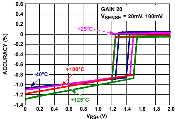
FIGURE 45. GAIN ACCURACY vs V_{RS+} = 0V TO 2V
