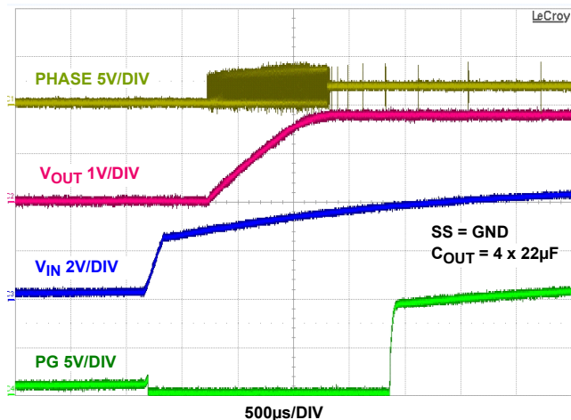
FIGURE 17. V_{\text{IN}} START-UP AT NO LOAD (SYNC = GND)
