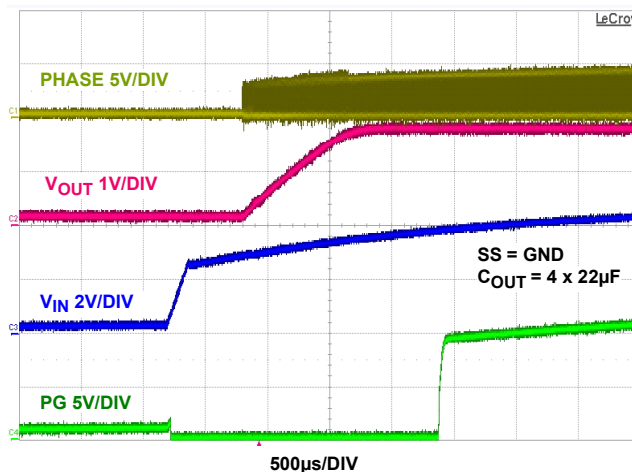
FIGURE 18. V_{\text{IN}} START-UP AT NO LOAD (SYNC = VDD)
