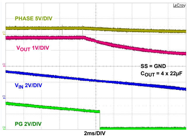
FIGURE 21. V_{\text{IN}} SHUTDOWN AT NO LOAD (SYNC = GND)
