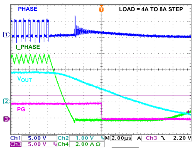
FIGURE 39. OVERCURRENT PROTECTION
