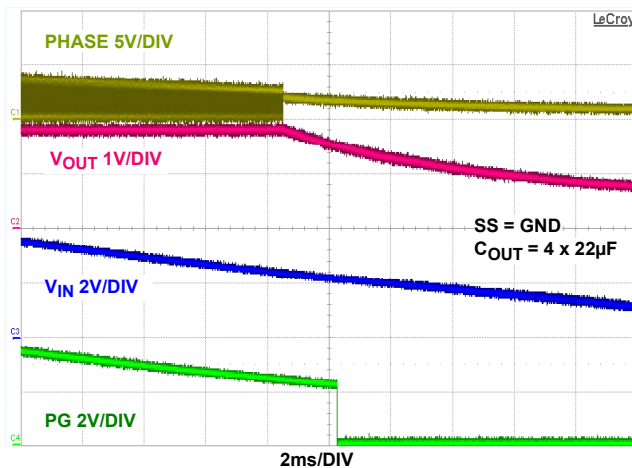
FIGURE 22. V_{\text{IN}} SHUTDOWN AT NO LOAD (SYNC = VDD)
