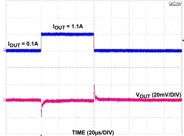
FIGURE 25. 1A LOAD TRANSIENT RESPONSE
