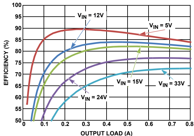
FIGURE 12. EFFICIENCY vs LOAD, PWM, V_{OUT} = 1.8V
