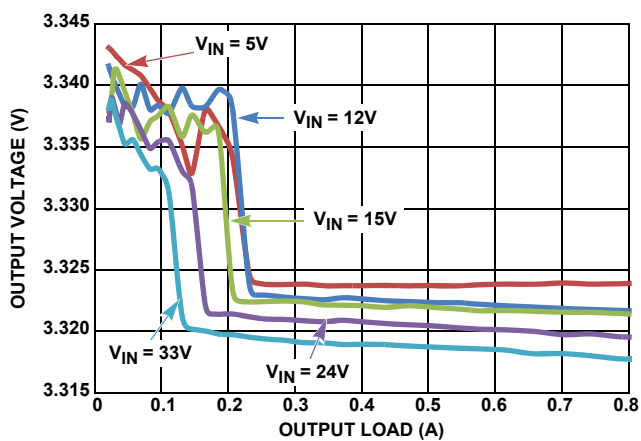
FIGURE 16. V_{OUT} REGULATION vs LOAD, PFM, V_{OUT} = 3.3V
