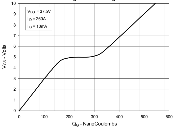
Fig. 9. Gate Charge
