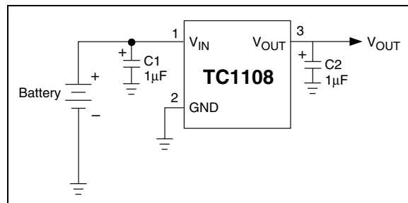
FIGURE 3-1: TYPICAL APPLICATION CIRCUIT
