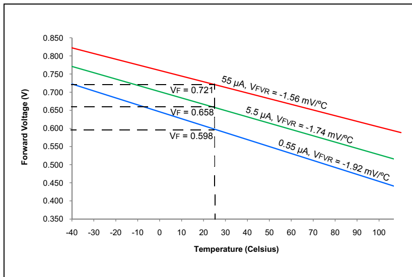
FIGURE 30-8: TYPICAL CTMU TEMPERATURE DIODE FORWARD VOLTAGE
