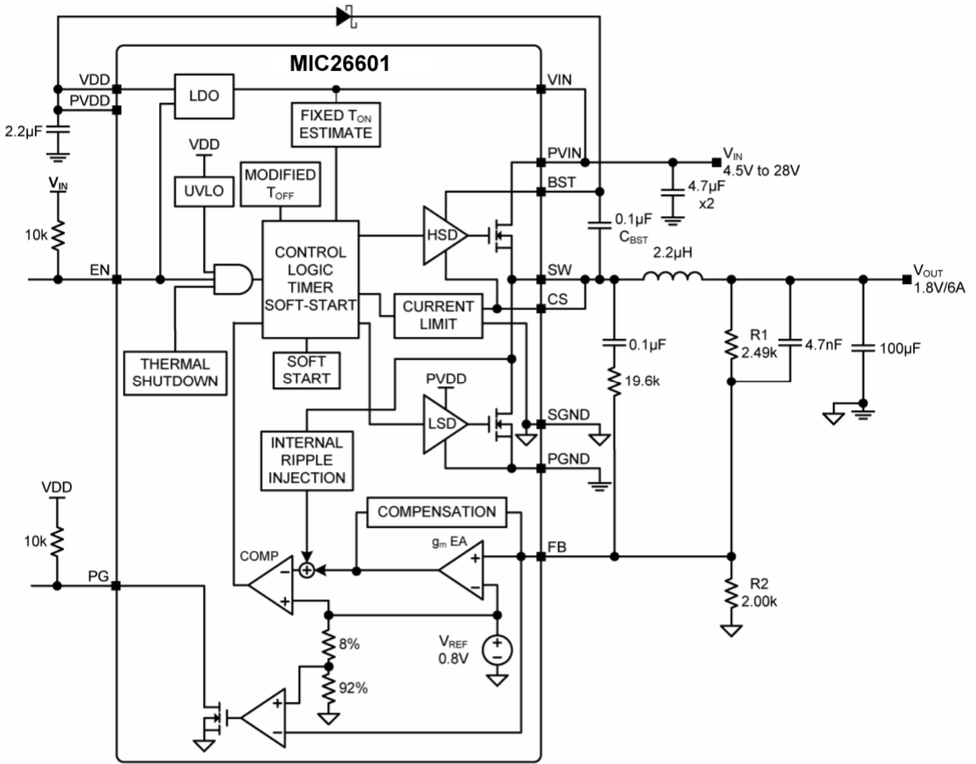
Figure 1. MIC26601 Block Diagram
