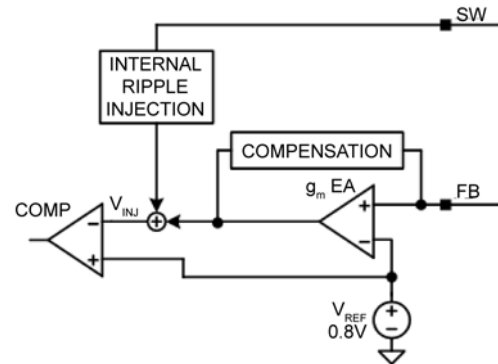
Figure 7. Internal Ripple Injection
