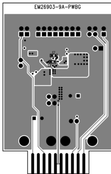
Figure 12. MIC26601 Evaluation Board Bottom Layer
