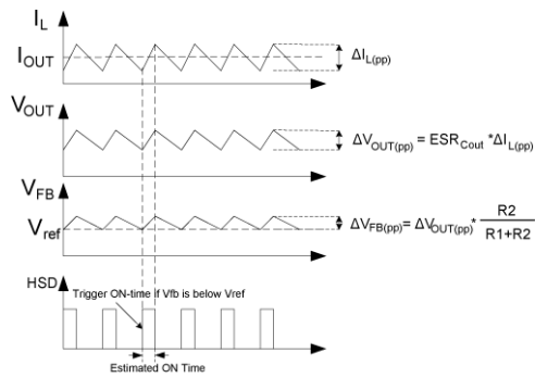
Figure 2. MIC26601 Control Loop Timing
