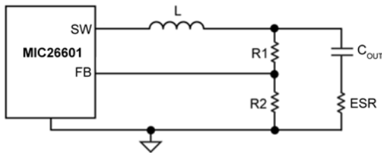
Figure 5a. Enough Ripple at FB
