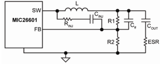
Figure 5c. Invisible Ripple at FB
