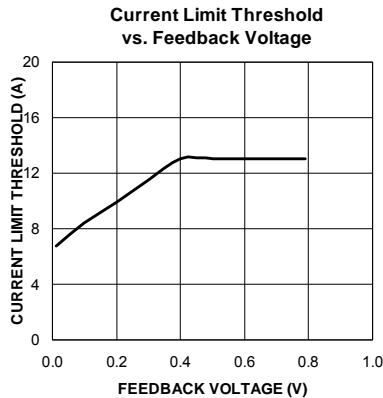
Figure 4. MIC26601 Current-Limit Foldback Characteristic
