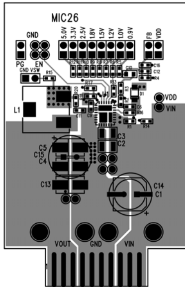
Figure 9. MIC26601 Evaluation Board Top Layer
