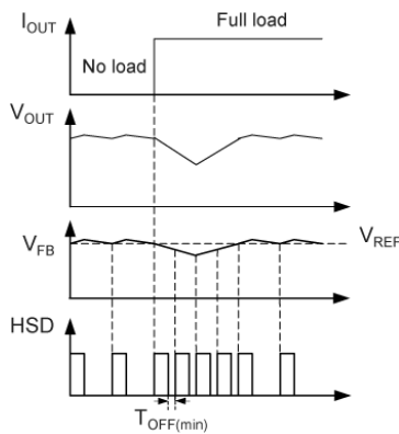
Figure 3. MIC26601 Load Transient Response
