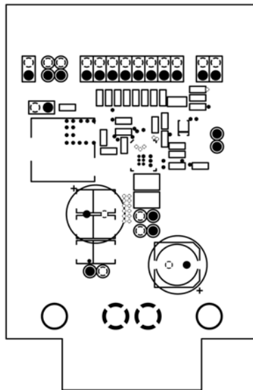
Figure 10. MIC26601 Evaluation Board Mid-Layer 1 (Ground Plane)
