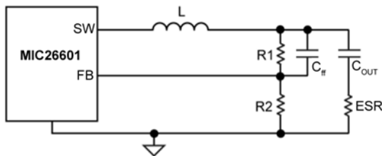
Figure 5b. Inadequate Ripple at FB
