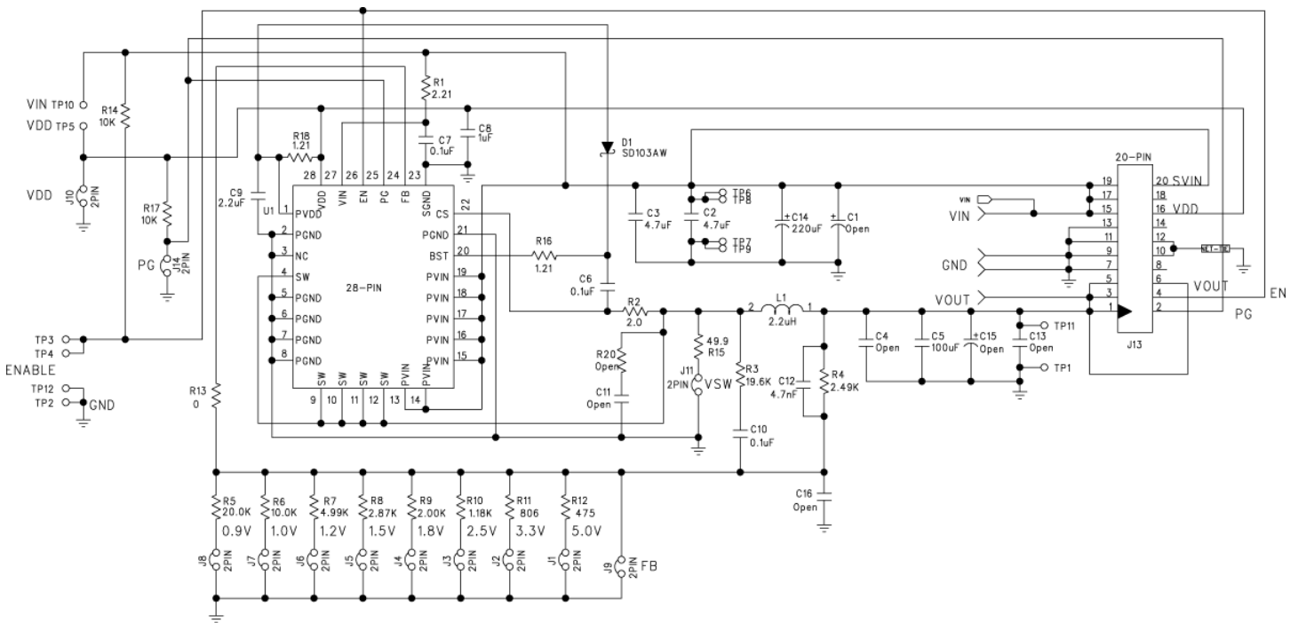
Figure 8. Schematic of MIC26601 Evaluation Board
