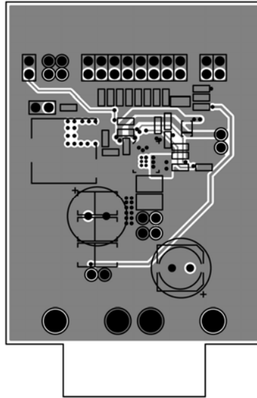
Figure 11. MIC26601 Evaluation Board Mid-Layer 2
