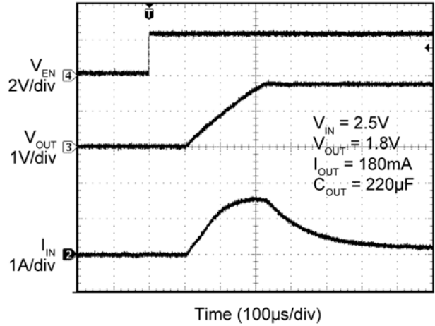
Inrush Current, C_{OUT} = 220\mu F
