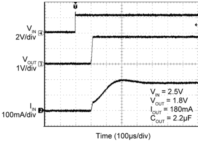
Inrush Current, C_{OUT} = 2.2\mu F
