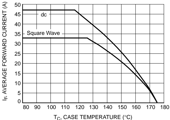
Figure 5. Current Derating for MBR60L45CTG
