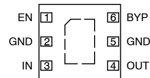
DFN6 (Top View)
