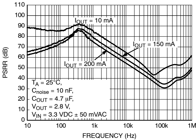
Figure 16. PSRR vs. Frequency, 2.8 V Output Voltage Option, C_{OUT} = 4.7 \mu\text{F} , C_{noise} = 10 \text{ nF}
