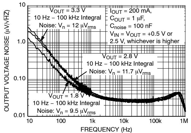
Figure 21. Output Noise vs. Frequency, C_{OUT} = 1 \mu\text{F} , C_{noise} = 100 \text{ nF} , I_{OUT} = 200 \text{ mA}
