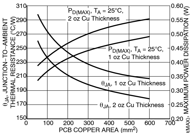
Figure 57. Thermal Resistance and Maximum Power Dissipation vs. Copper Area (TSOP-5)
