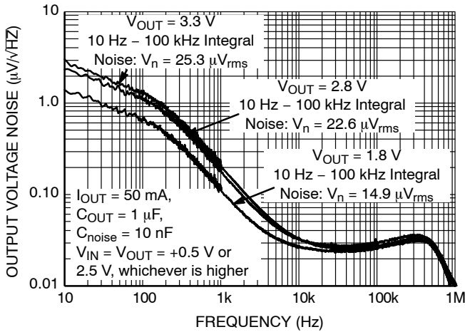
Figure 18. Output Noise vs. Frequency, C_{OUT} = 1 \mu\text{F} , C_{noise} = 10 \text{ nF} , I_{OUT} = 50 \text{ mA}
