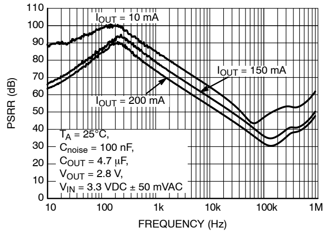
Figure 17. PSRR vs. Frequency, 2.8 V Output Voltage Option, C_{OUT} = 4.7 \mu\text{F} , C_{noise} = 100 \text{ nF}
