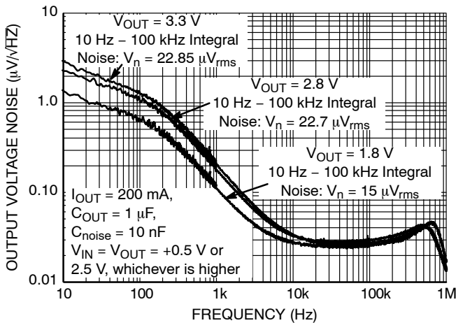
Figure 20. Output Noise vs. Frequency, C_{OUT} = 1 \mu\text{F} , C_{noise} = 10 \text{ nF} , I_{OUT} = 200 \text{ mA}
