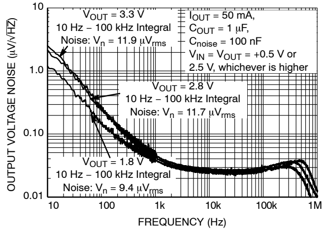
Figure 19. Output Noise vs. Frequency, C_{OUT} = 1 \mu\text{F} , C_{noise} = 100 \text{ nF} , I_{OUT} = 50 \text{ mA}
