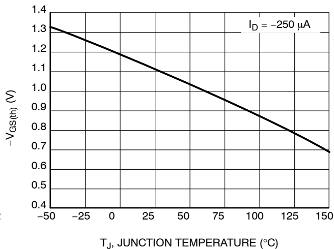
Figure 21. Threshold Voltage
