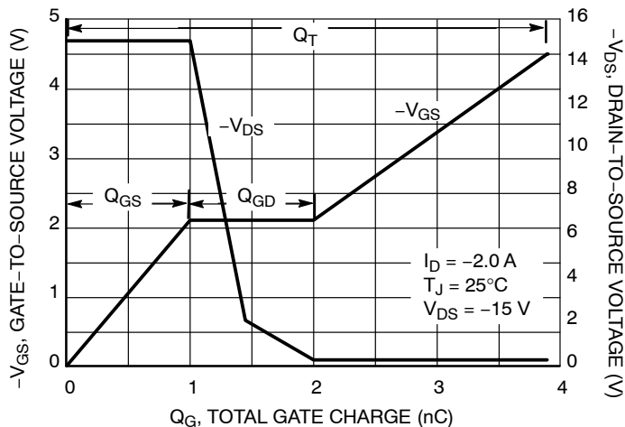
Figure 19. Gate-to-Source and Drain-to-Source Voltage versus Total Charge
