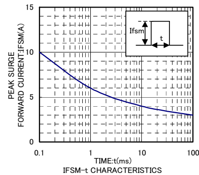
IFSM-t CHARACTERISTICS
