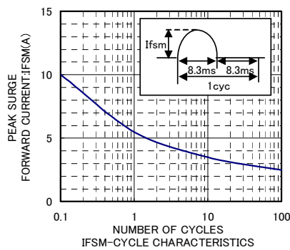
IFSM-CYCLE CHARACTERISTICS
