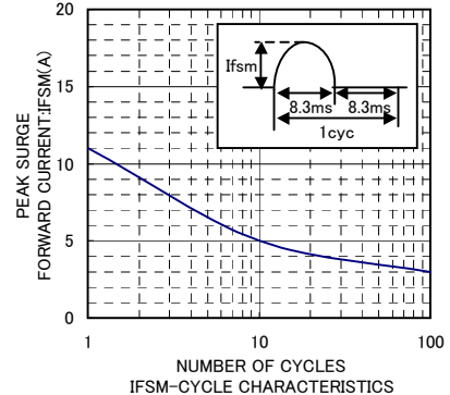
IFSM-CYCLE CHARACTERISTICS
