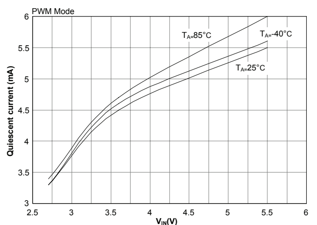
Quiescent Current vs. Input Voltage, PWM Mode
