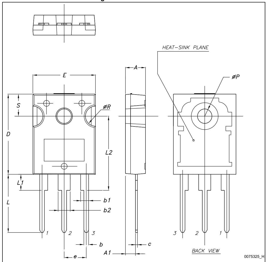
Figure 32. TO-247 outline
