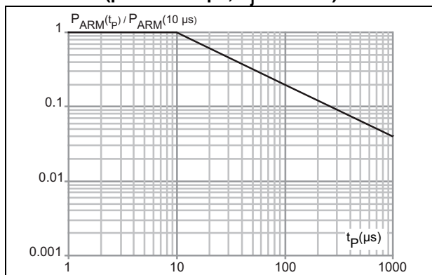
Figure 3. Normalized avalanche power derating versus pulse duration (pulse > 10 \mu s, T_j < 150 °C)
