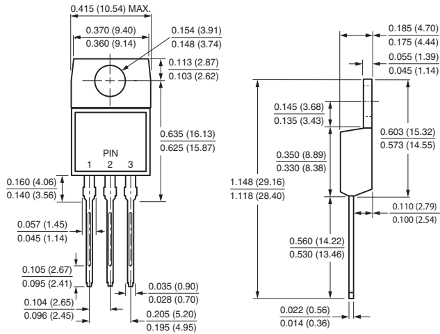
TO-220AB
